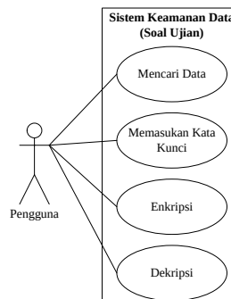
Gambar 4 Use Case Diagram
