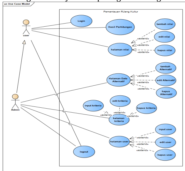
Gambar 2. Usecase Diagram
