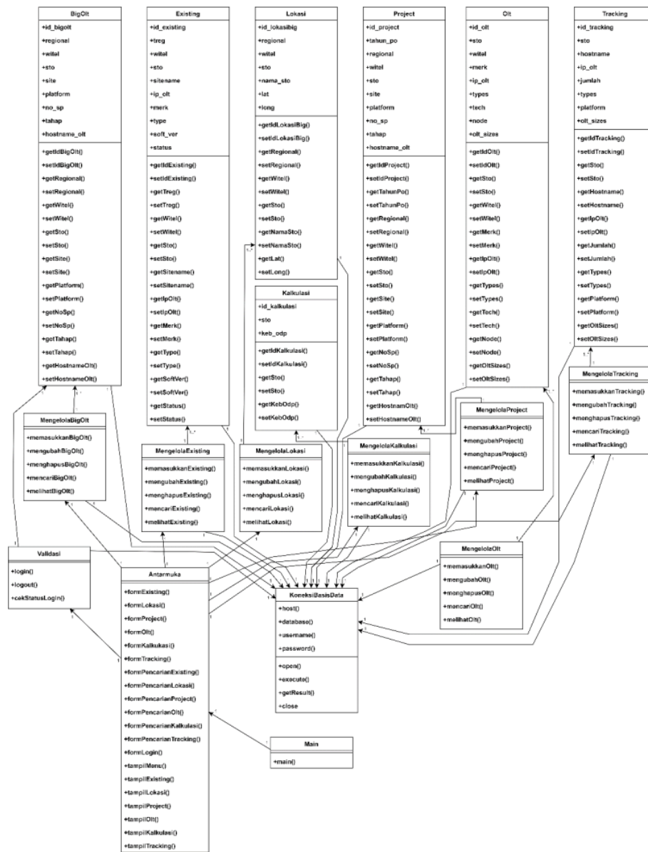
Gambar 4. Rancangan class diagram
